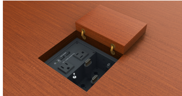
Cable Cubby 650 UT open – Compatible with Series/2 power modules, AAPs, Extron Retractors, and cables.
