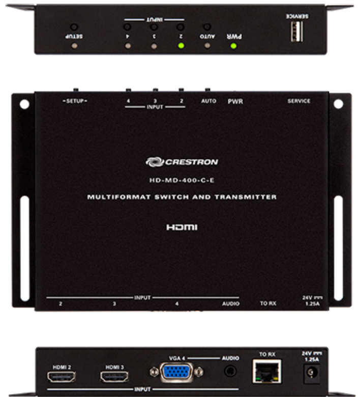
HD-MD-400-C-E Transmitter – Top, Front, and Bottom Views
